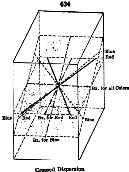
Crossed Dispersion
